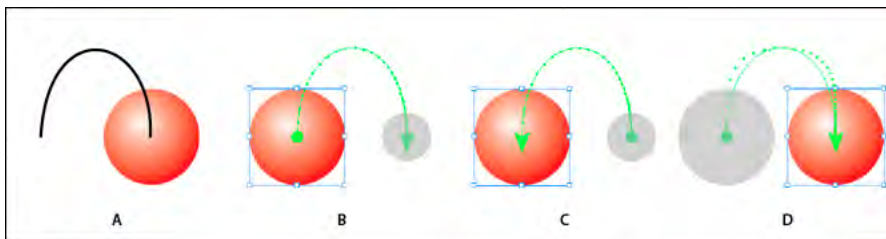
Animate settings
