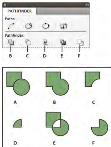
Pathfinder panel
